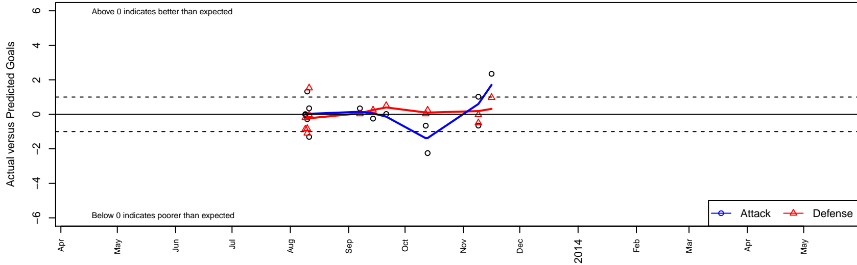
Placer United 03 Red B02 Dots are actual minus expected GF (blue circles) and GA (red triangles). Blue line is smoothed change in attack strength. Red is smoothed change in defense strength.
